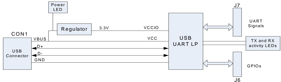
Figure 4-2. Hardware Block Diagram
